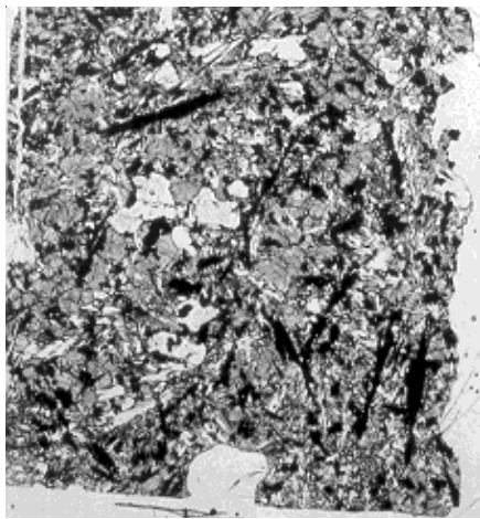
Figure 3a, b: Thin section photos showing abundant, platy ilmenite in 71055.
