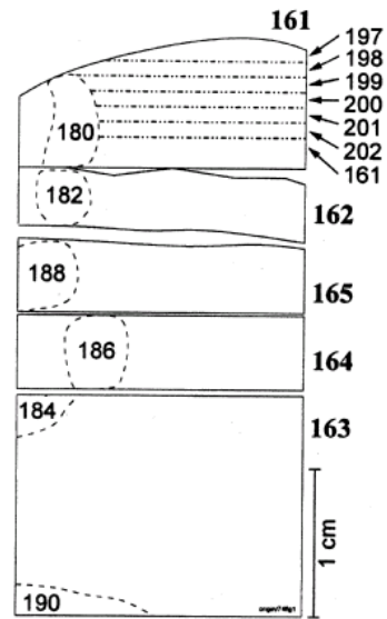
Figure 13: Schematic drawing of column cut from 74275 for study of cosmogenic radionuclide production from energetic solar cosmic ray (from Fink et al. 1998).
