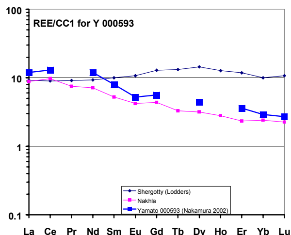
Figure XXII-3: Normalized rare earth element diagram comparing data from Yamato 000593 with Nakhla and Shergotty (data from Nakamura et al. 2002).
