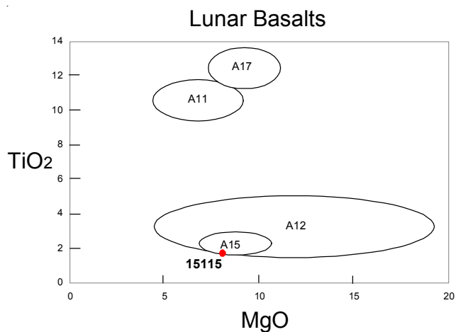
Figure 3: Chemical composition of 15115 compared with other Apollo basalts.
