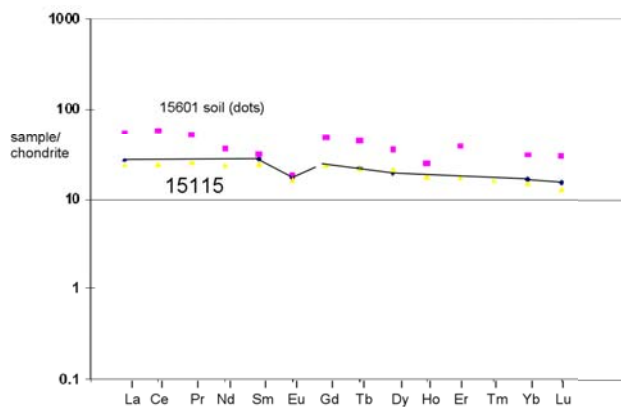
Figure 4: Normalized rare-earth-element diagram for 15115, with 15601 soil for comparison.
