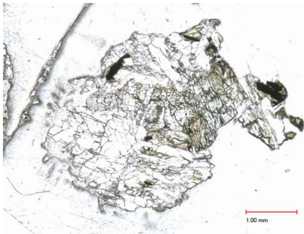
Figure 2a: Photomicrograph of 15117,2 by C Meyer @ 50x.
