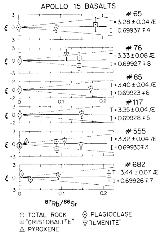
Figure 5: Rb/Sr isochrons for Apollo 15 basalts including 15117 (from Papanastassiou and Wasserburg 1973).
