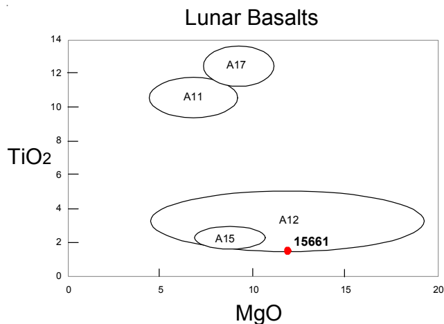
Figure 3: Chemical composition of 15661 compared with other Apollo basalts.
