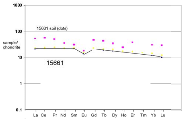
Figure 4; Normalized rare-earth-diagram for 15661, with soil 15601 for comparison.
