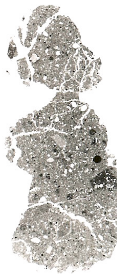
Figure 3: Photomicrograph of thin section 74115,14 - about 1 cm.
