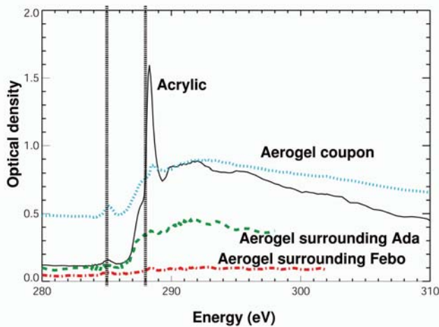
Fig. 14. Four C-XANES spectra are shown. The spectrum labeled “aerogel coupon” corresponds to a piece of bulk aerogel (courtesy of A. Butterworth). The spectrum labeled “acrylic” corresponds to a microtomed section of aerogel embedded in acrylic in which the acrylic has not been removed using chloroform. The spectrum labelled “aerogel surrounding Ada” corresponds to a section of the particle Ada surrounded by aerogel and embedded in acrylic, which was washed with chloroform and the acrylic dissolved. The spectrum labelled “aerogel surrounding Febo” corresponds to a section of the particle Febo surrounded by aerogel and embedded in acrylic, which was washed with chloroform and the acrylic dissolved. The spectrum labelled “acrylic” is dominated by a sharp, high peak at 288.5 eV that is absent in the other three spectra. Instead, the spectra of the aerogel have a small, broader peak at 288.5 eV. All four spectra have a small peak at 285 eV.
