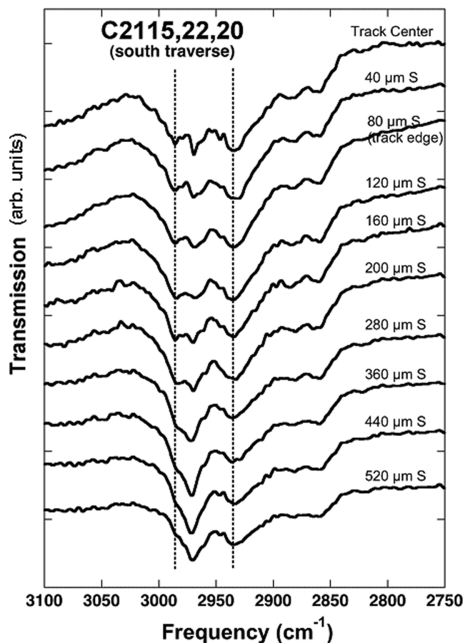
Fig. 3. Details of infrared spectra taken from track C2115,22,20. The spectra were taken every 40\text{ }\mu\text{m} starting from the track center and are displayed offset for better visibility. Dashed lines at 2985 and 2935\text{ cm}^{-1} mark spectral positions where excess absorption is seen as one approaches the center of the track. It is also clear that the material that produces these two bands is not restricted solely to the confines of the physical impact track, but instead extends outward beyond the nearest edge of the track (the physical edge of the track is at the 80\text{ }\mu\text{m S} position). A similar dispersion is seen on both sides of the track.
