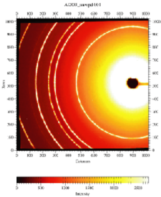
SRM-674a \alpha -corundum
