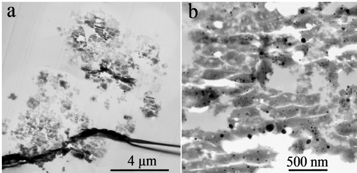
Fig. 2. a) Low-magnification bright-field TEM image showing an entire slice in C2054,0,35,51,3. The vitreous matrix (dark gray) appears discontinuous. The black curved linear features are due to sample preparation. b) STEM bright-field image showing the typical microstructure of the shard-like silica-rich glass matrix in the samples that contains variable but minor amounts of MgO, Al 2 O 3 , and/or CaO and has numerous opaque metal and sulfide inclusions dispersed in variable sizes and number distributions (sample C2004,1,44,4,2).
