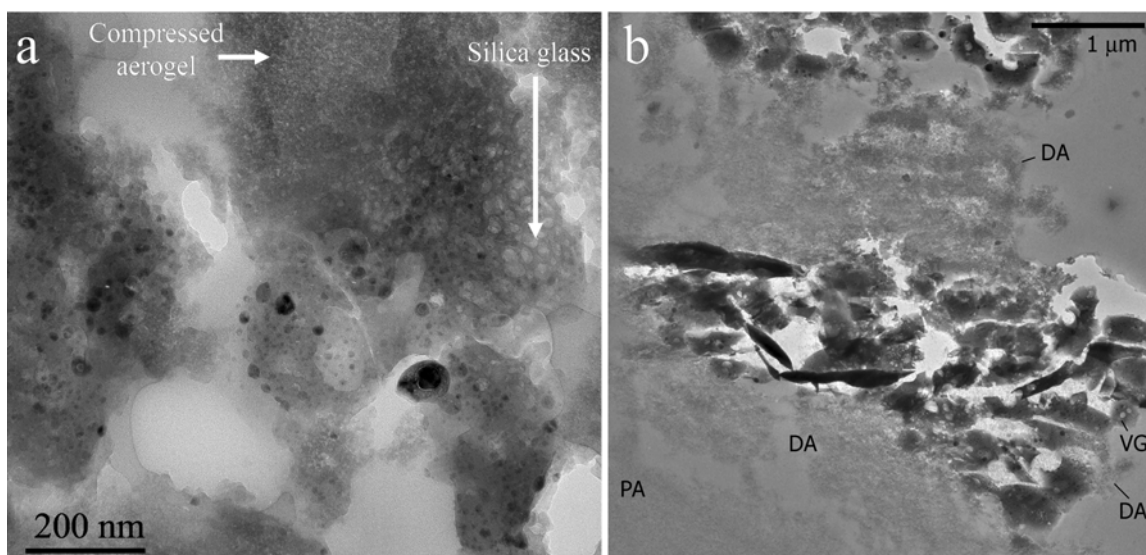
Fig. 4. Bright-field TEM images. a) Glassy matrix with high concentrations of opaque inclusions, compressed aerogel, and highly vesicular, pure silica glass (sample C044,2,41,3,4). b) Discontinuous glassy matrix in sample C2054,0,35,16,1, showing that the aerogel texture varies from fully pristine (PA) to densified (DA) to melted vesicular glass (VG). The uniform light to dark gray areas is the embedding medium used to prepare the ultra-thin sections. The irregular white areas are probably due to loss of sample material. The dark angular shards consist of glass.
