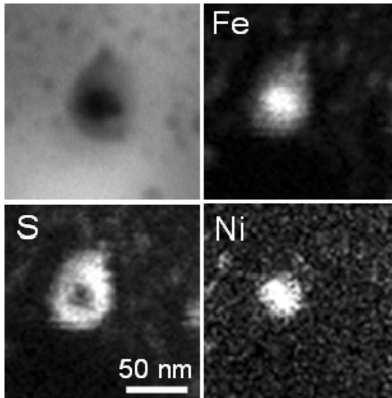
Fig. 8. EDS intensity distribution for Fe, S, and Ni of a large core/mantle inclusion in FC3,0,2,2,1. The metallic core that contains ~3 at% Ni is surrounded by an iron sulfide rim with a Fe:S ratio close to 1:1 at%.
