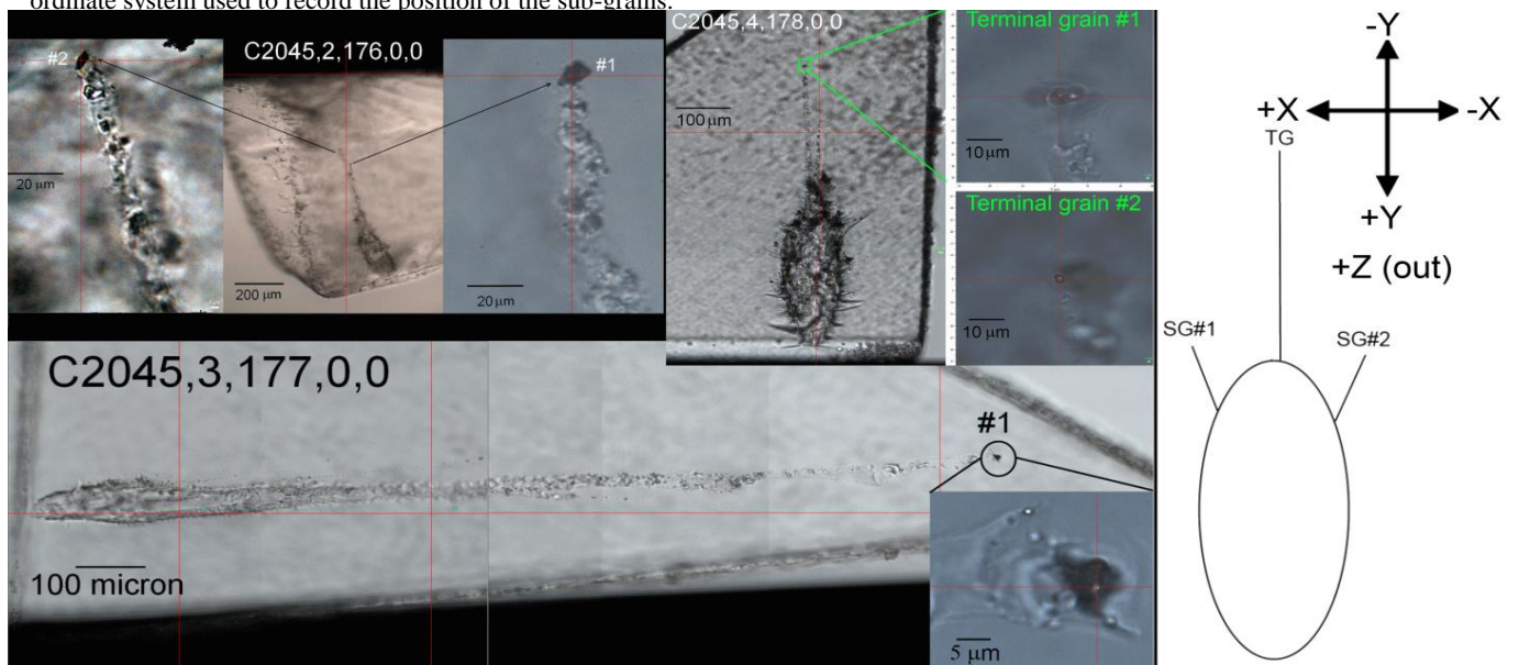
Figure 1 (below): Images of tracks 176, 177, 178 showing the position of the main terminal grains. The right hand sketch gives the coordinate system used to record the position of the sub-grains.
